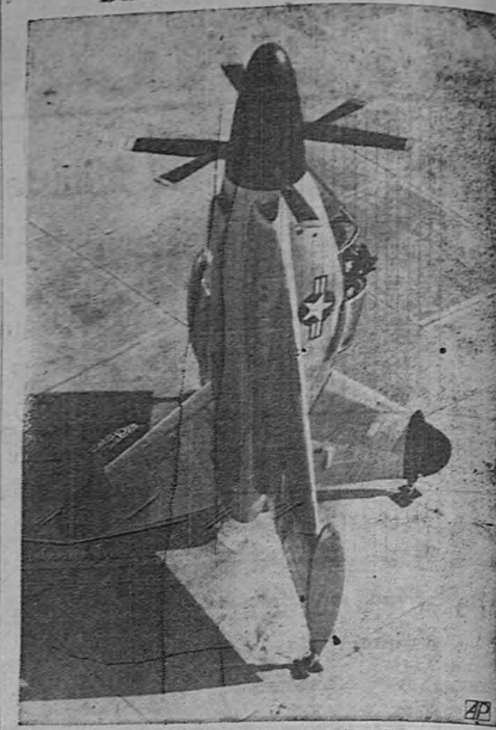
The Navy's new Convair "XFY-1" vertical takeoff delta-wing fighter, rests on its tail with its nose pointed straight up. The plane is designed to take off and land in this position. A similar vertical takeoff plane has been built by Lockheed. This photo was made available by the Navy in Washington, March 15.
